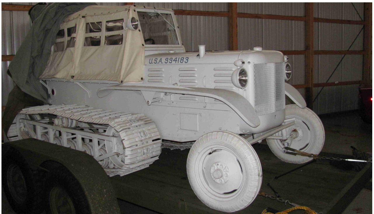
M7 Snow Tractor – Jaap Rietveld Collection (Belgium)
