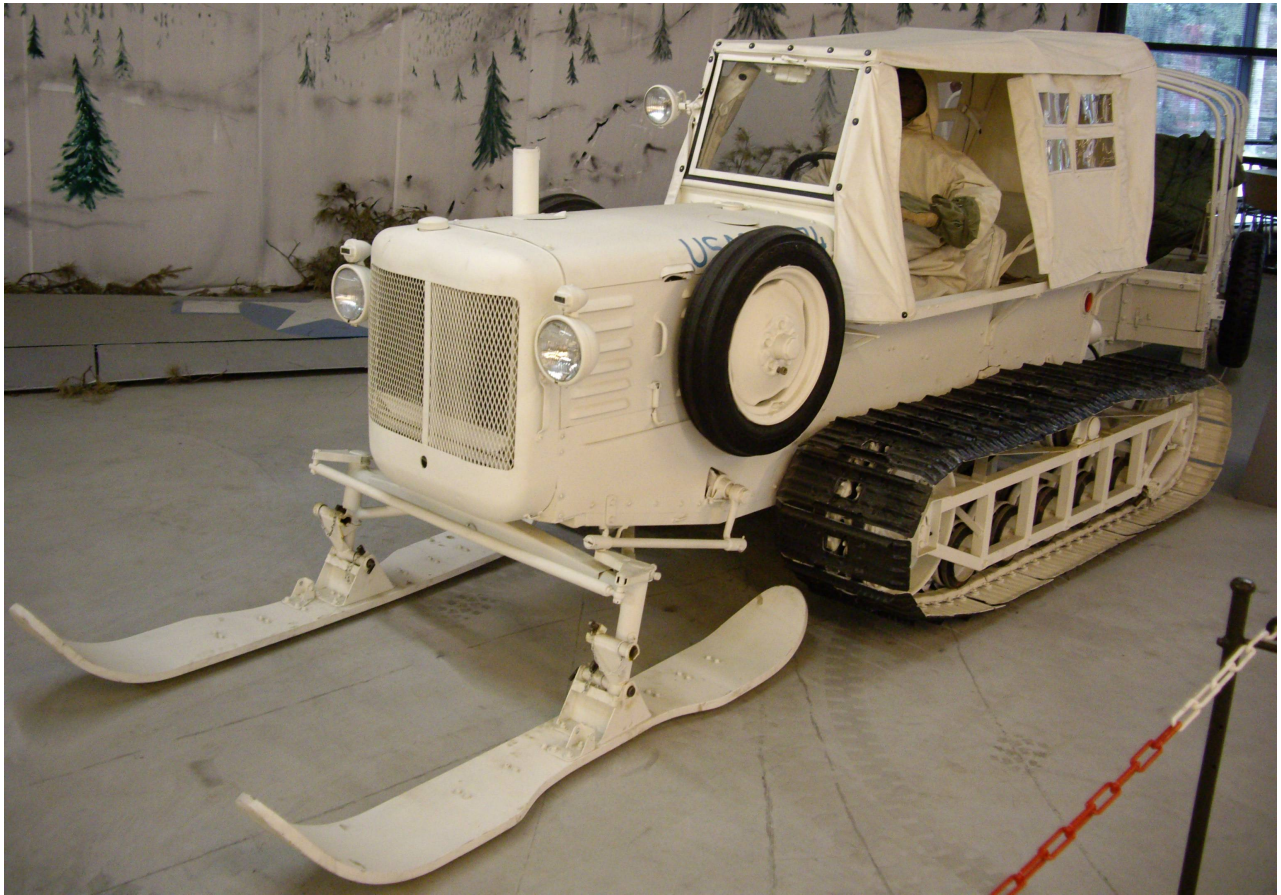
M7 Snow Tractor – National War and Resistance Museum Overloon (Netherlands)
