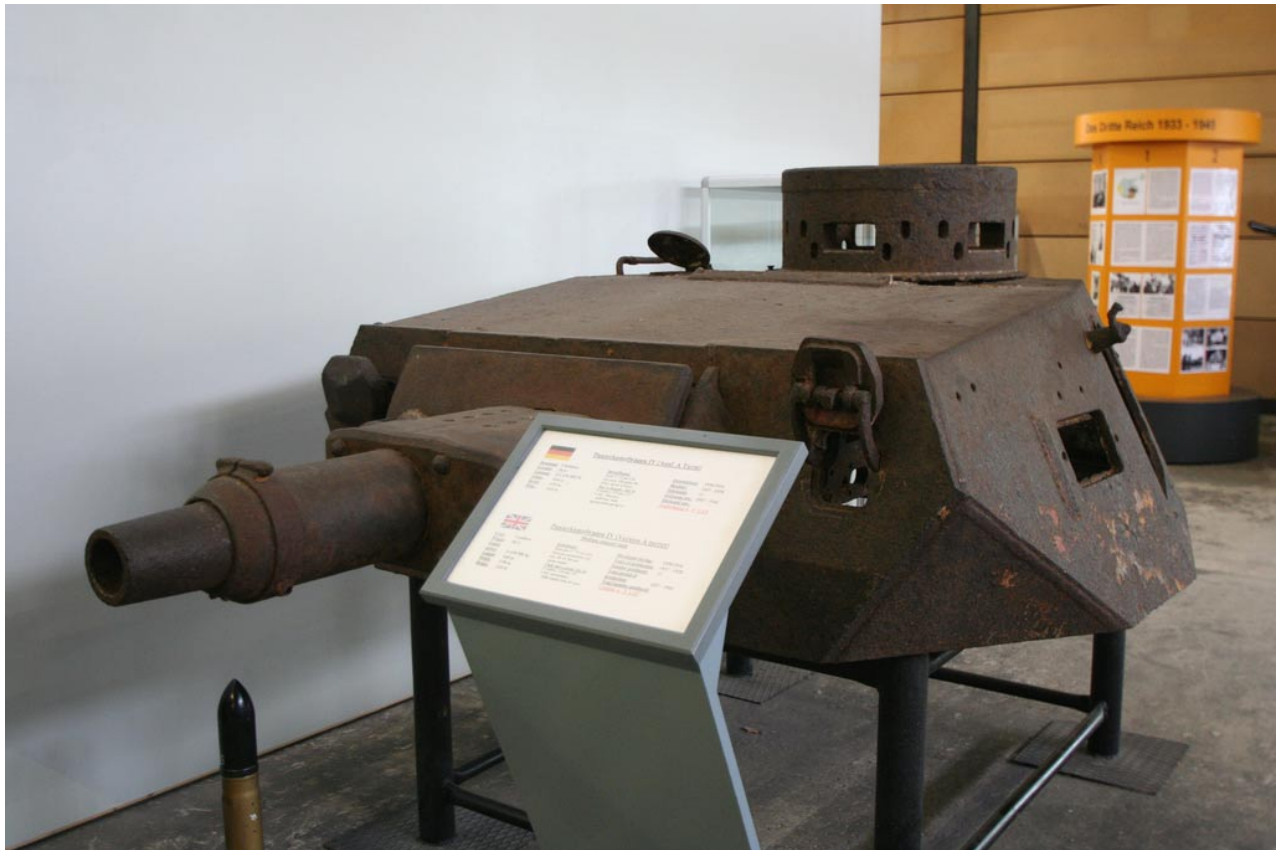
PzKpfw. IV Ausf. D turret – Munster Panzer Museum (Germany)
