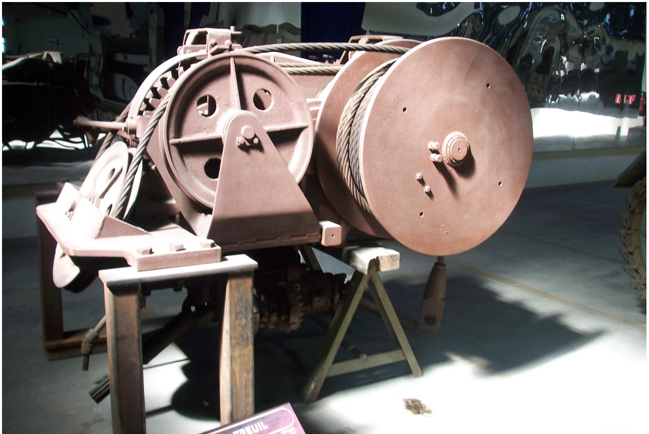
Bergepanther crane mechanism – Saumur Tank Museum (France)
