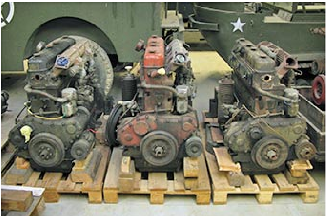
Three Jagdpanzer 38(t) Hetzer engines – ASPHM Association, La Wantzenau (France)
